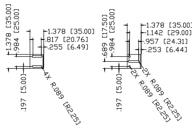
BRACKET DETAIL
